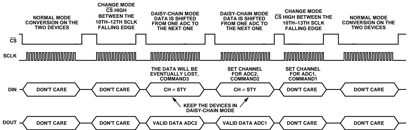
Figure 34. Daisy-Chain Diagrams—1
