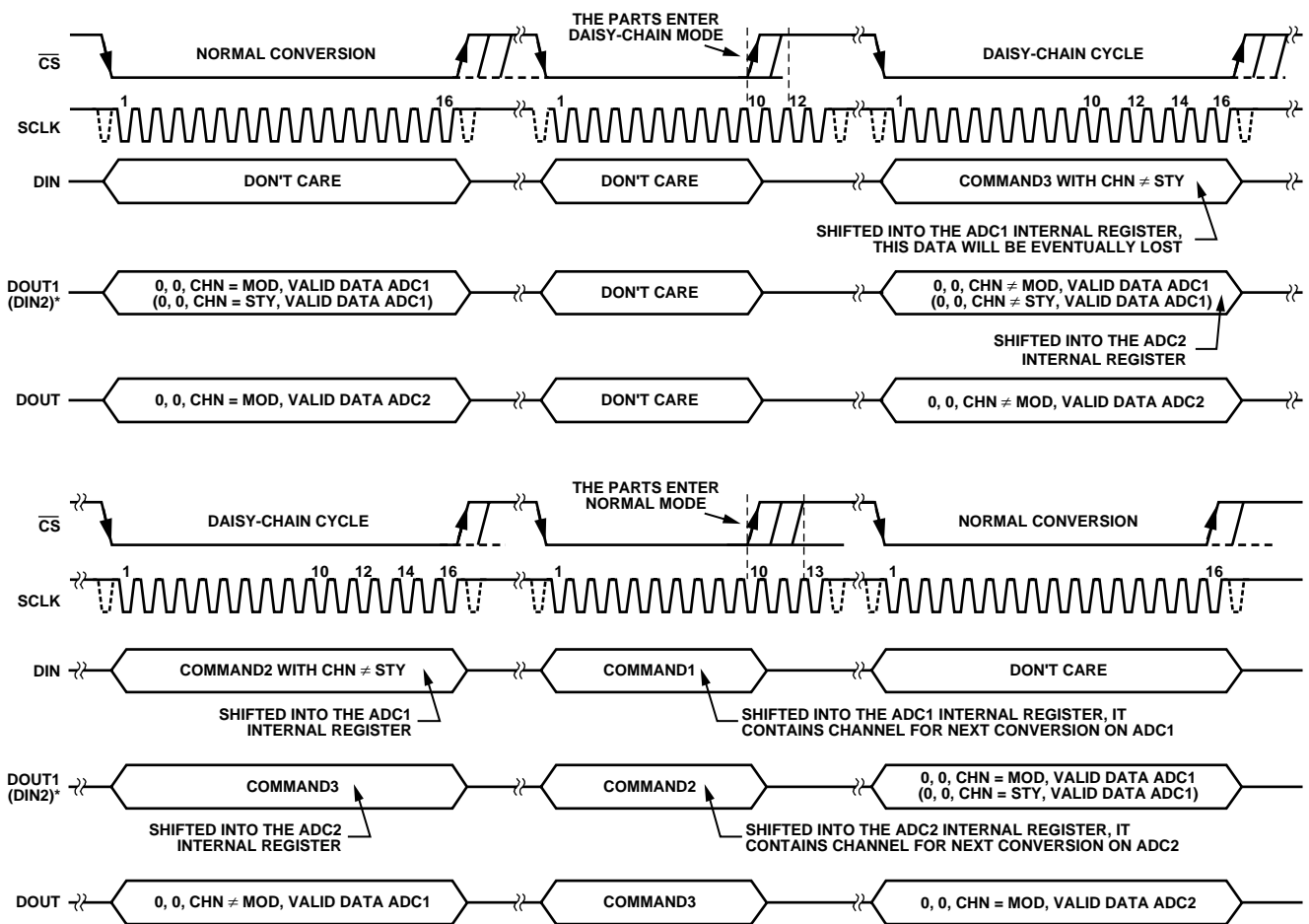
Figure 35. Daisy-Chain Diagrams—II
