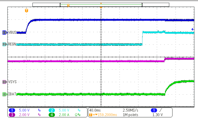
图 51. Power Up with Charge Enabled
