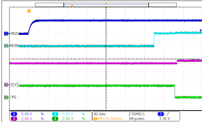
图 50. Power Up with Charge Disabled
