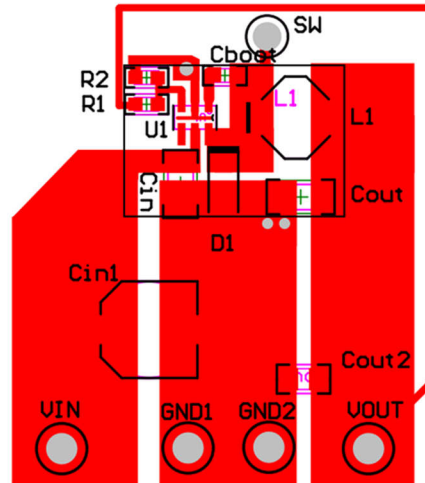
Figure 8-9. Layout Example
