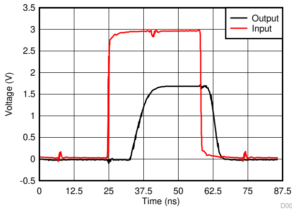
图 7-3. Switching Characteristics at 15 MHz Excellent Signal Integrity
