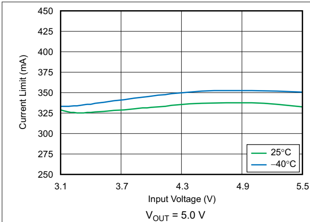
图 6-31. Current Limit vs Input Voltage
