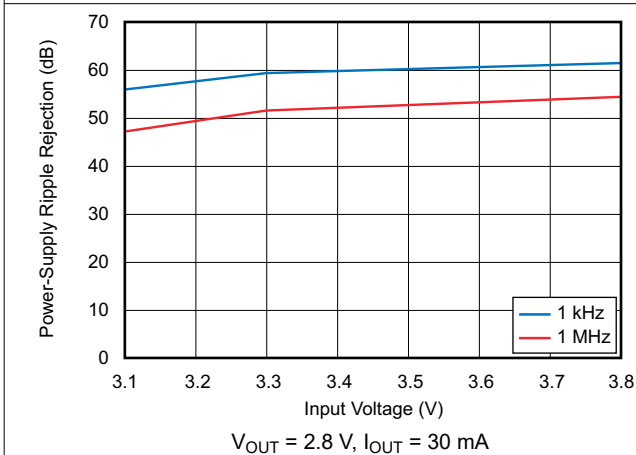
图 6-35. Power-Supply Ripple Rejection vs Input Voltage
