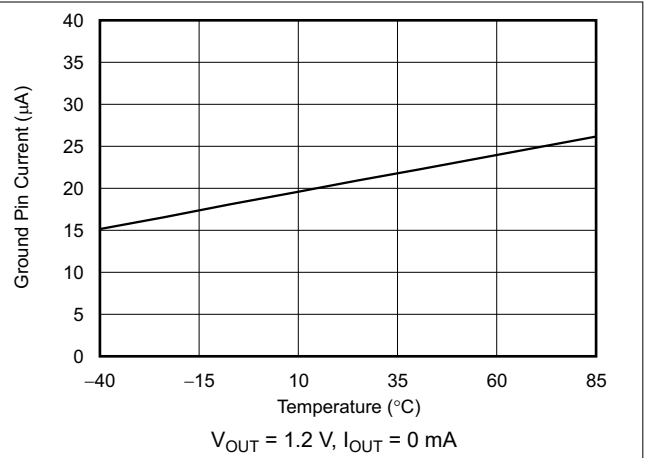
图 6-20. Ground Pin Current vs Temperature
