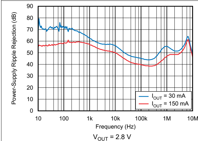
图 6-33. Power-Supply Ripple Rejection vs Frequency
