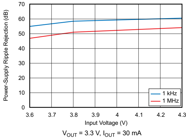
图 6-37. Power-Supply Ripple Rejection vs Input Voltage
