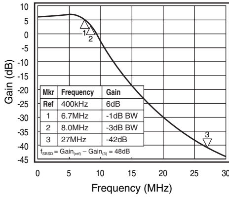
Figure 3. Frequency Response
