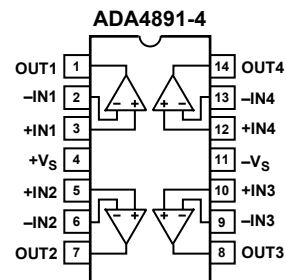
Figure 5. 14-Lead SOIC_N (R-14) and 14-Lead TSSOP (RU-14)
