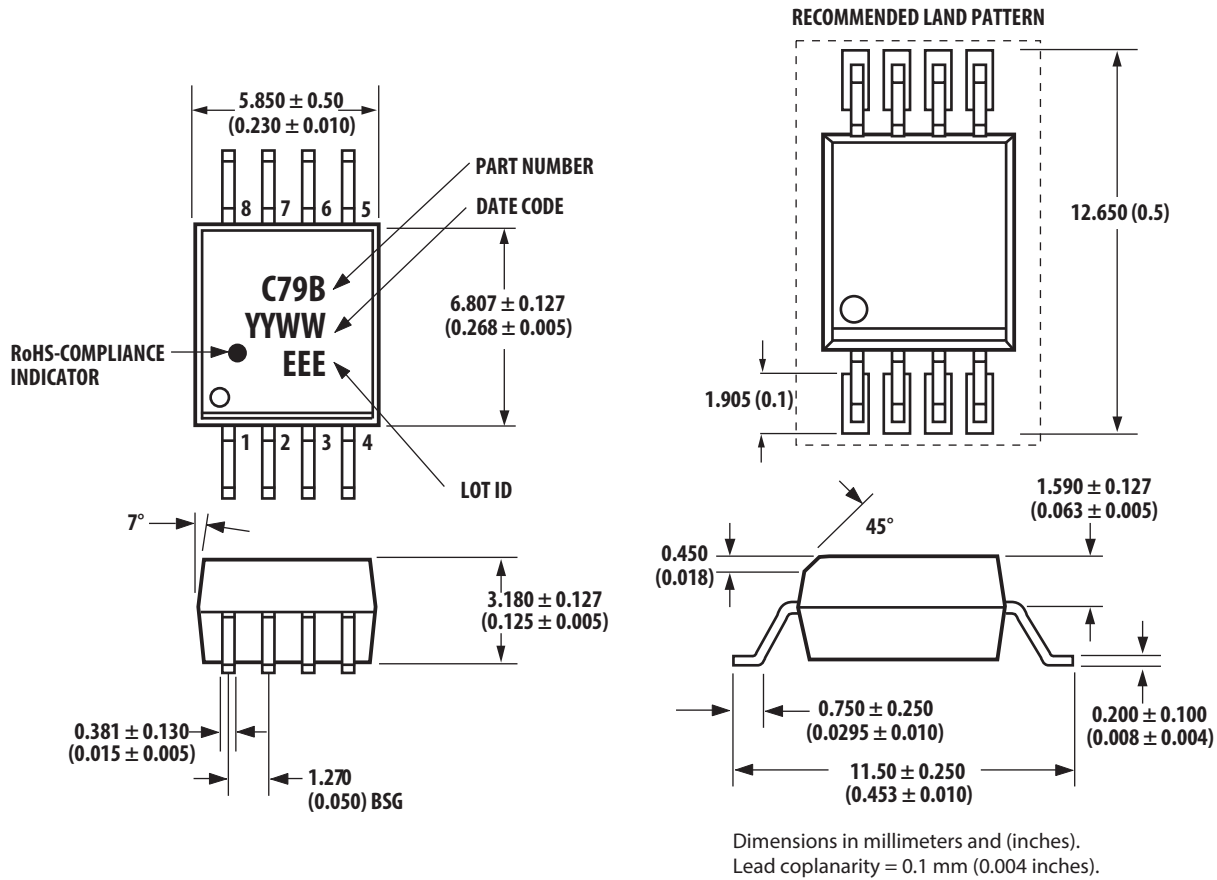
Figure 2. SSO-8 package.
