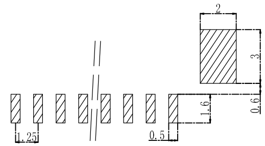
PCB尺寸 PCB Layout
