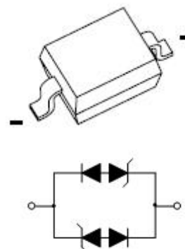
SOD-323
