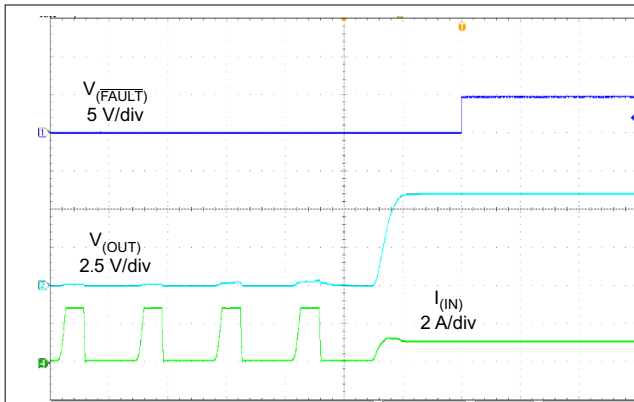
图 6-24. Short-Circuit to Full-Load Recovery
