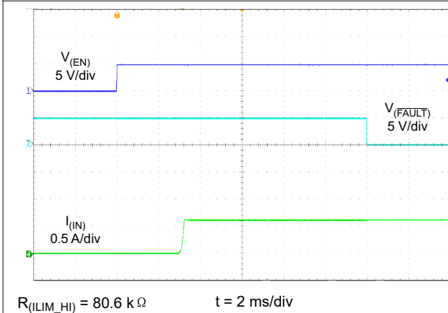
图 6-22. Enable Into Short
