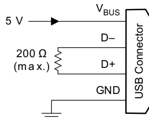
图 8-8. DCP Supporting BC1.2 and YD/T 1591-2009
