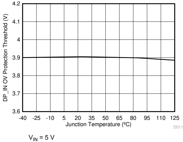
图 6-11. DP_IN Overtolerance Protection Threshold vs Temperature
