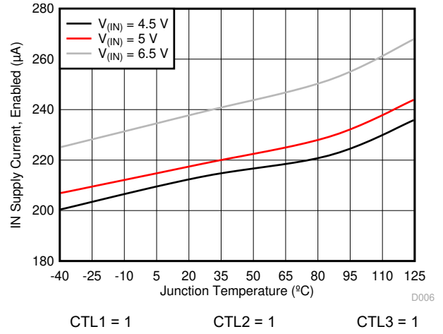
图 6-6. Enabled IN Supply Current - CDP (111) vs Temperature
