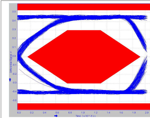
图 6-18. Eye Diagram Using USB Compliance Test Pattern, Bypassing the TPS2549-Q1 Data Switch
