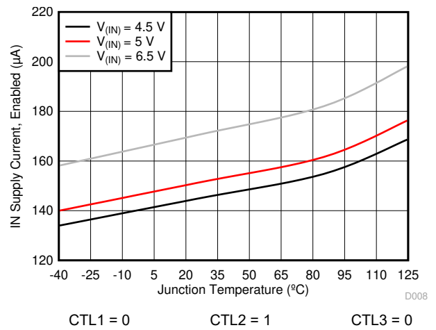
图 6-8. Enabled IN Supply Current - SDP (010) vs Temperature
