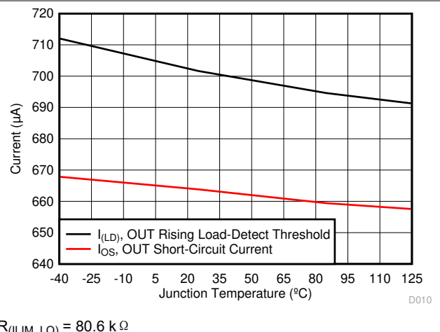
图 6-10. I OUT Rising Load-Detect Threshold and OUT Short-Circuit Current Limit vs Temperature
