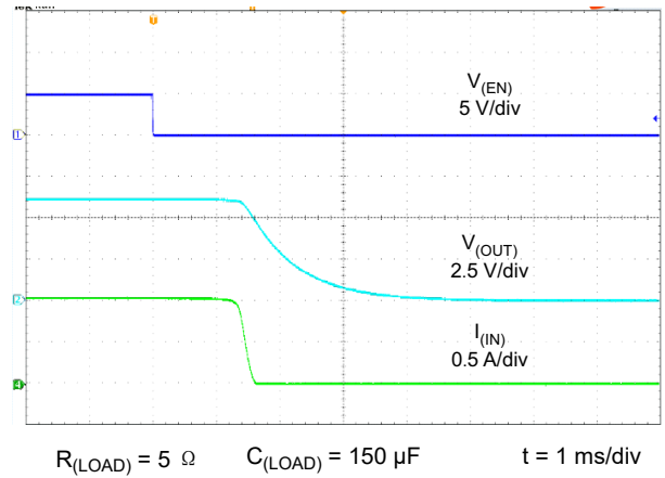
图 6-21. Turnoff Response
