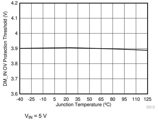
图 6-12. DM_IN Overtolerance Protection Threshold vs Temperature
