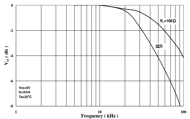
Figure 18. Frequency Response
