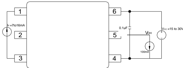
Figure 14 : V_{OH} Test Circuit
