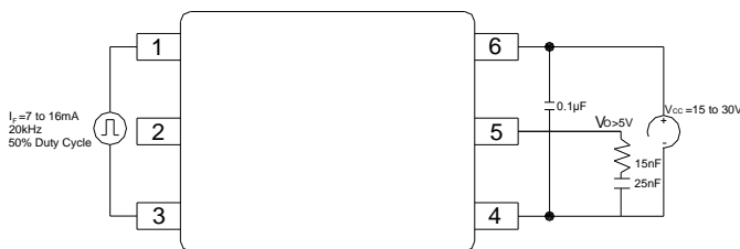
Figure 20 : t_r , t_f , t_{PLH} and t_{PHL} Test Circuit and Waveforms
