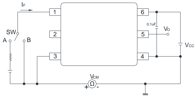
Figure 21 : CMR Test Circuit and Waveforms
