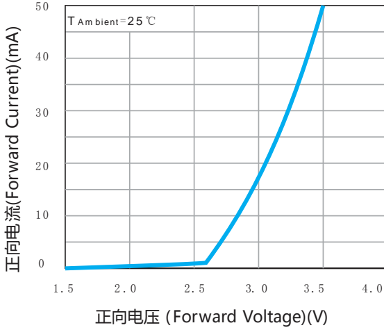
Volt-Ampere Characteristics
