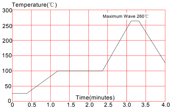
FIG.6: Lead-free profile
