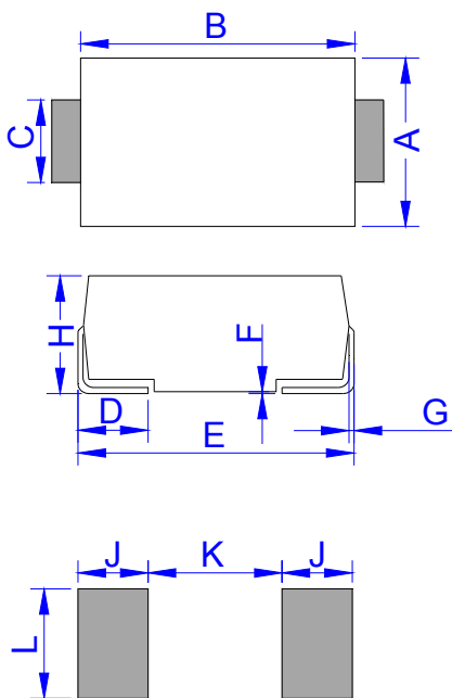
DO-214AA (SMB)
