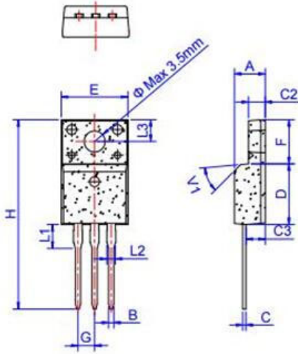
TO-220F
