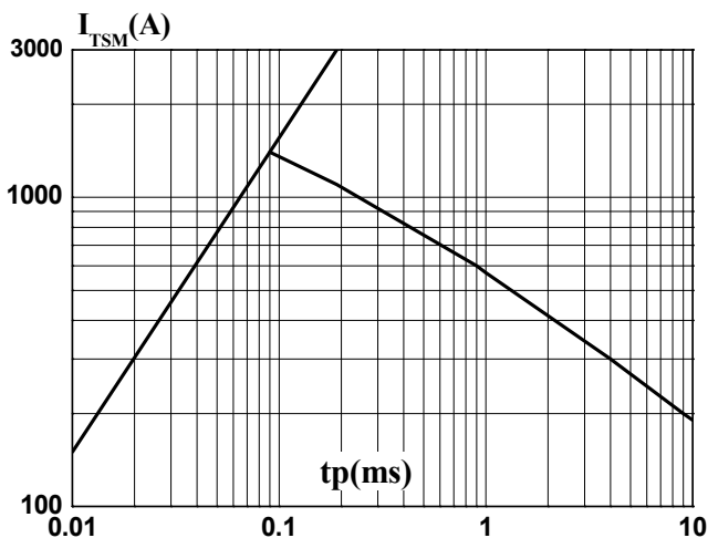
FIG.5: Non-repeating peak surge current vs. sine wave pulse width relationship graph
