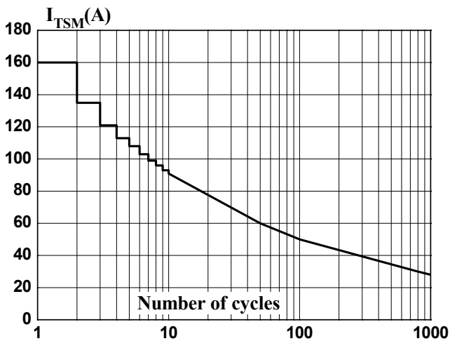
FIG.3: Peak surge current vs. number of cycles graph
