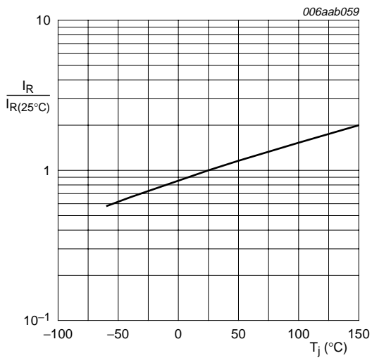
PESD5Z2.5; V RWM = 2.5 V PESD5Z3.3; V RWM = 3.3 V I R is less than 50 nA at 150 °C for: PESD5Z5.0; V RWM = 5.0 V PESD5Z6.0; V RWM = 6.0 V PESD5Z7.0; V RWM = 7.0 V PESD5Z12; V RWM = 12.0 V
