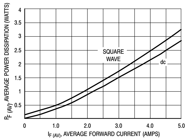
Figure 4. Power Dissipation
