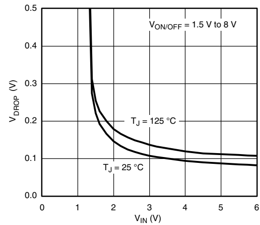
V_{DROP} vs. V_{IN} at I_L = 0.7 A
