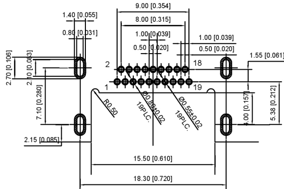
RECOMMENDED P.C.B LAYOUT (THICKNESS=1.2mm) (COMPONENT SIDE) TOLERANCES±0.05mm
