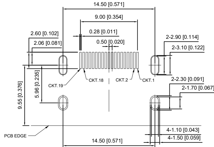
RECOMMENDED PCB LAYOUT CONNECTOR SIDE(TOP VIEW)
