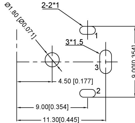
PCB HOLES(TOP VIEW) GENERAL TOLERAMCE:±0.1mm
