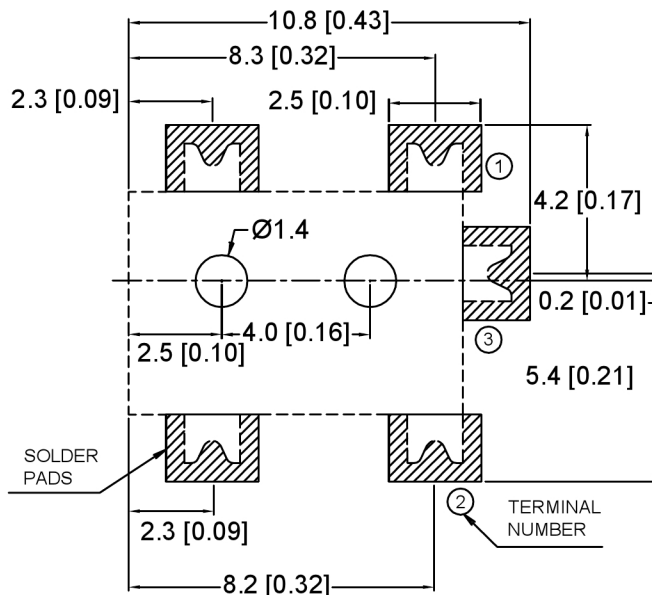
RECOMMENDED SOLDER PAD LAYOUT (TOP VIEW)
