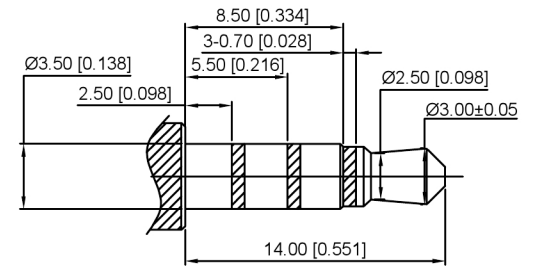
(Ø3.50mm 4 POLE PLUG DETAIL DRAWING)
