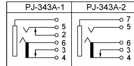
SCHMATIC
