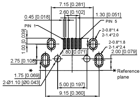
Recommended PCB Layout Tolerance:±0.1(Top view)
