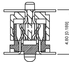
ASSEMBLY SCALE 2:1
