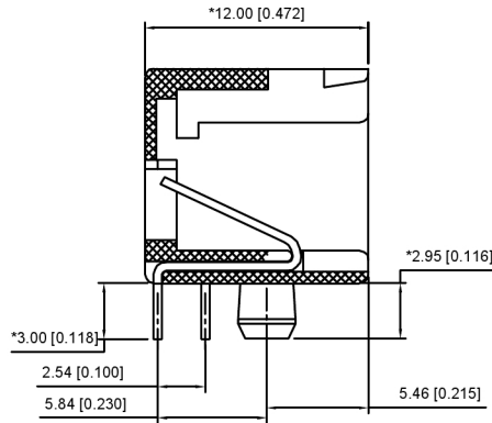
CUTAWAY VIEW
