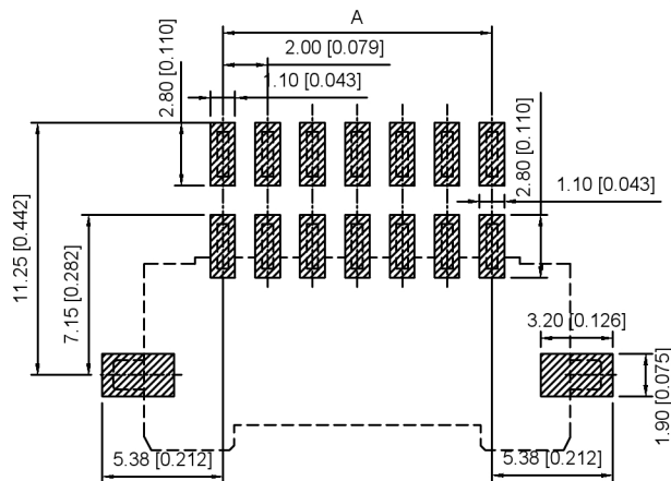
PCB LAYOUT(Tolerance:±0.05)
