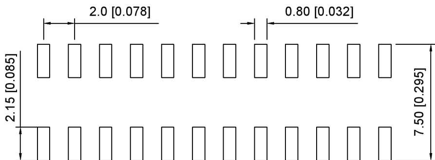
PCB LAYOUT
