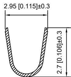
SECTION:A-A SCALE:1:1
