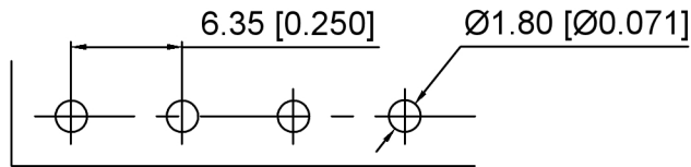
P.C.B board Layout
