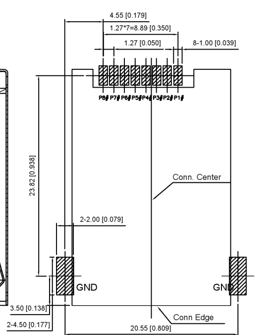
RECOMMENDED PCB LAYOUT (TOP VIEW) GENERAL TOLERANCES: ±0.05
